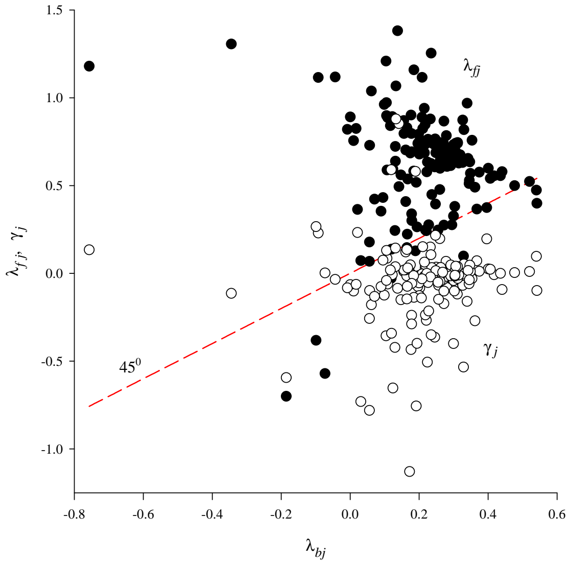
Figure 2: Coefficient Correlations
