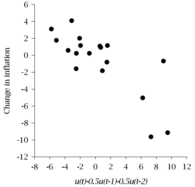
Phillips Curve: 1923-1940
